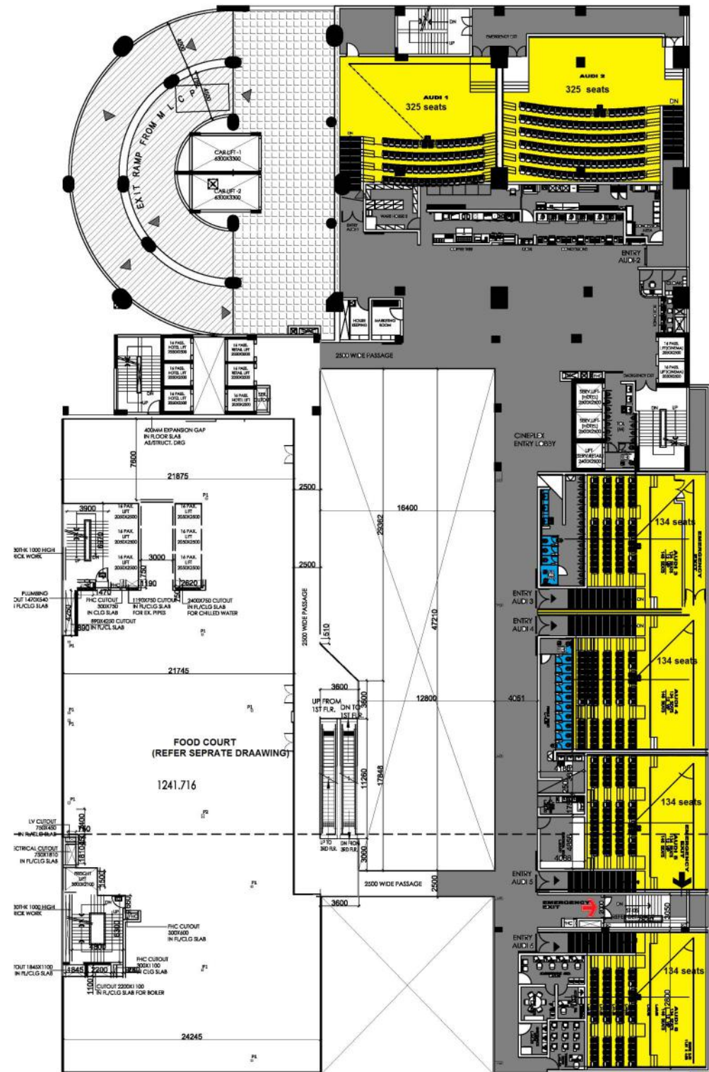
CINEMA ENTRY LEVEL FLOOR PLAN TOTAL 1186 SEATS TYPICAL FLOOR PLAN 2,3,4
