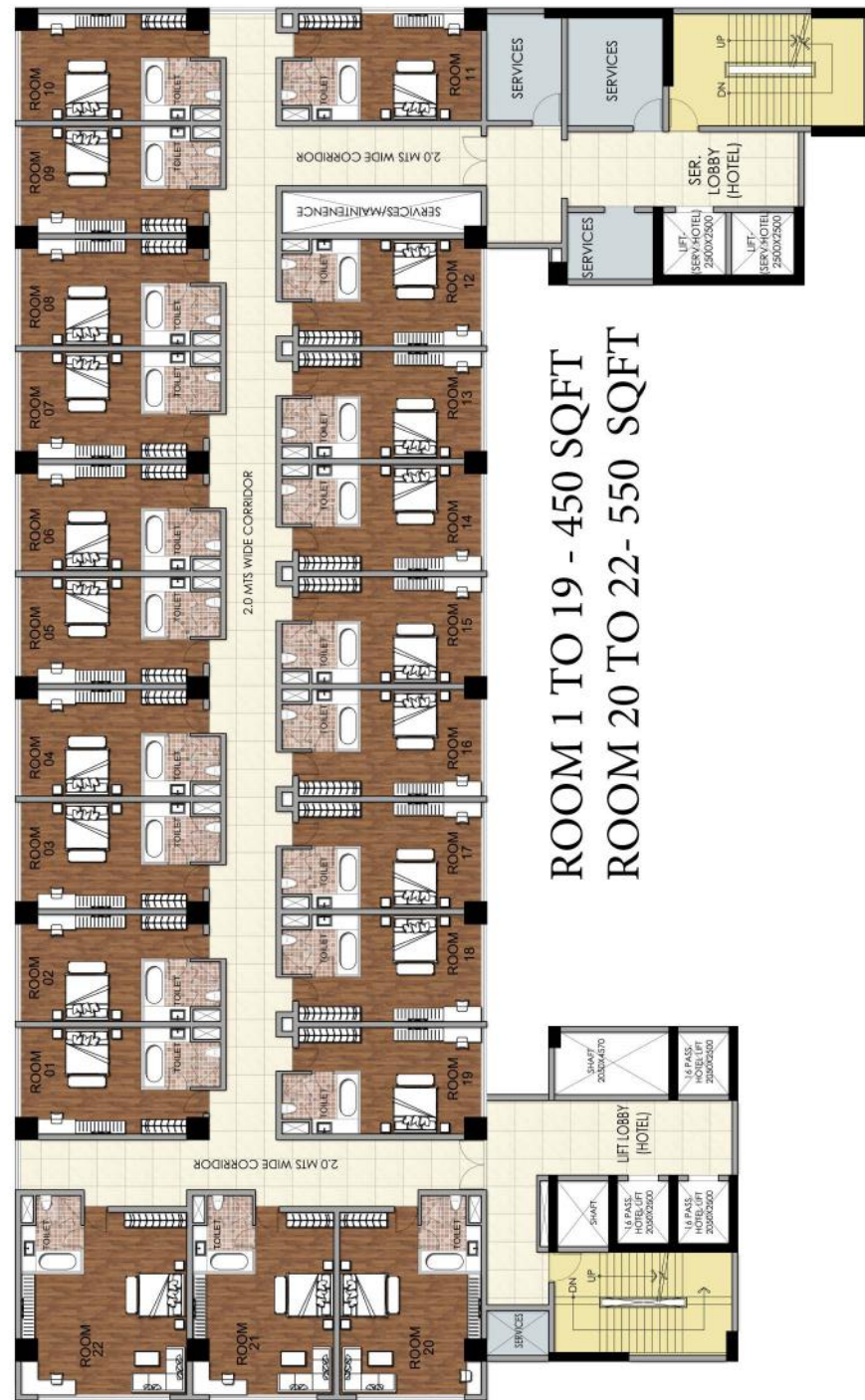
1HOTEL LEVEL FLOOR PLAN
